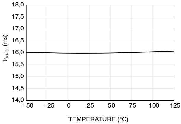
Figure 29. The Fault Timer Duration t_{fault}
