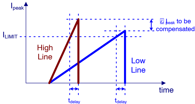
Figure 61. Needs for Line Compensation for True Overpower Protection
