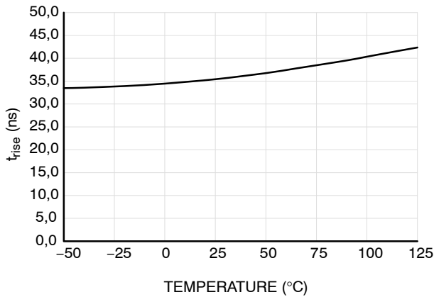
Figure 31. Output Driver Rise Time t_{rise}
