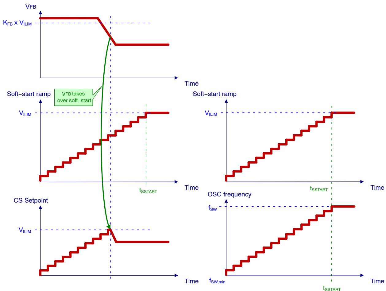
Figure 60. Soft-start Feature
